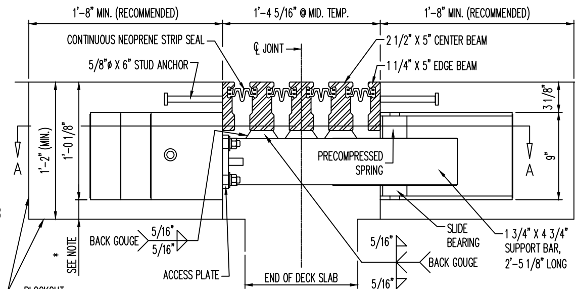
SECTION "B" - TYPICAL SECTION THROUGH 'D-320' EXPANSION JOINT @ SUPPORT BOX
