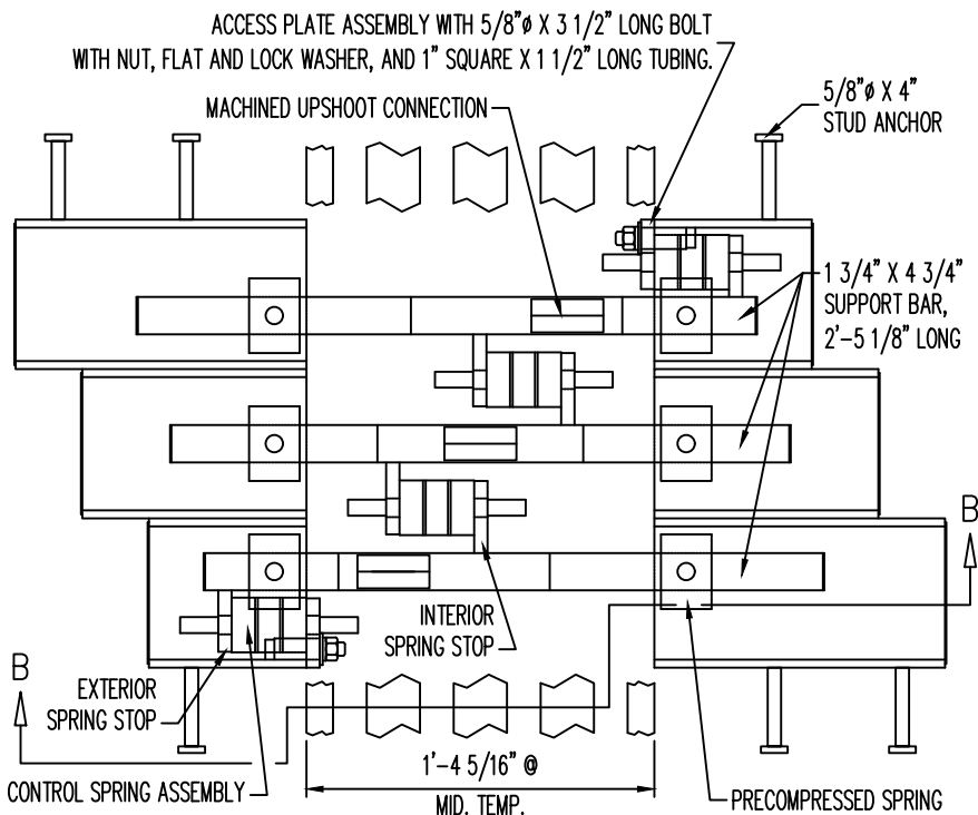
DETAIL "A" - PLAN VIEW OF 'D-320' EXPANSION JOINT @ SUPPORT BOX
