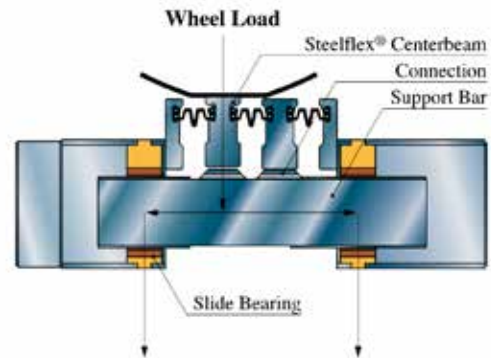
Wheel Load Transfer
